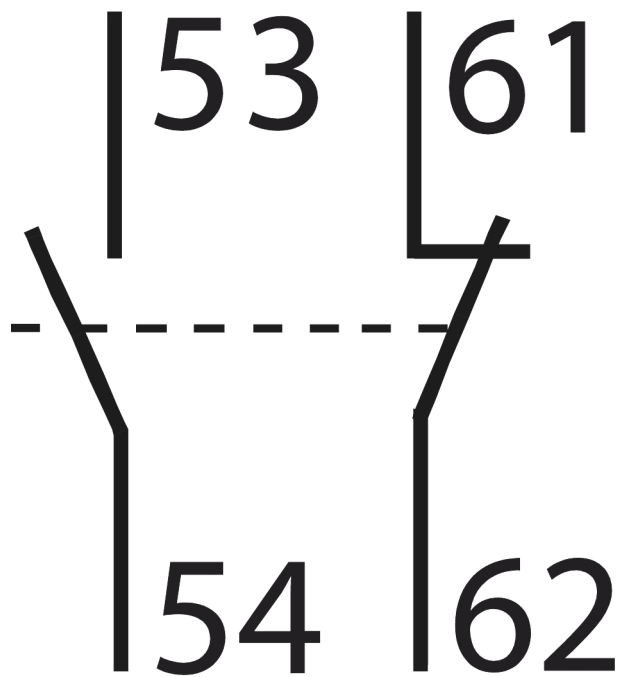
Connection / Wiring Diagram
