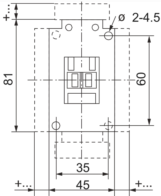
Dimension Diagram
