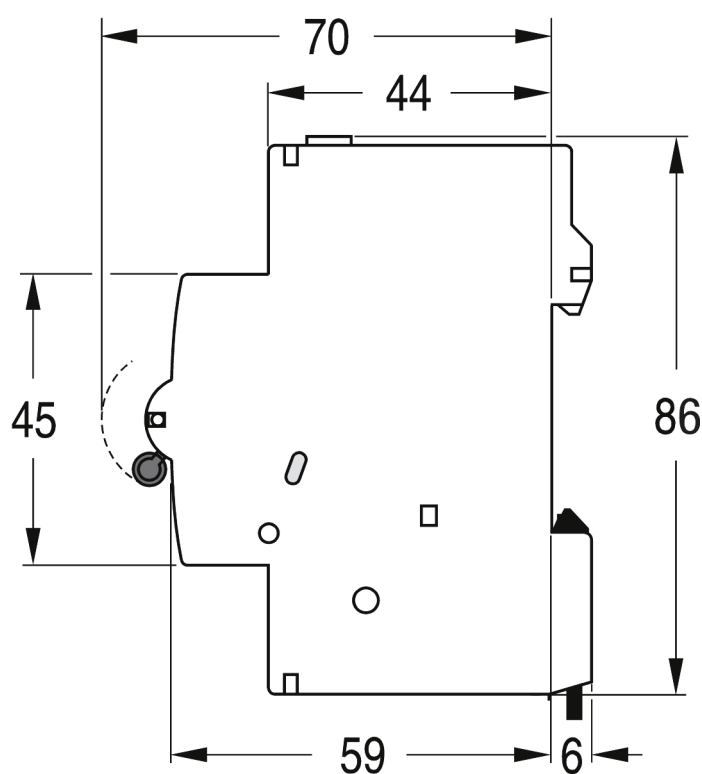
Dimension Diagram
