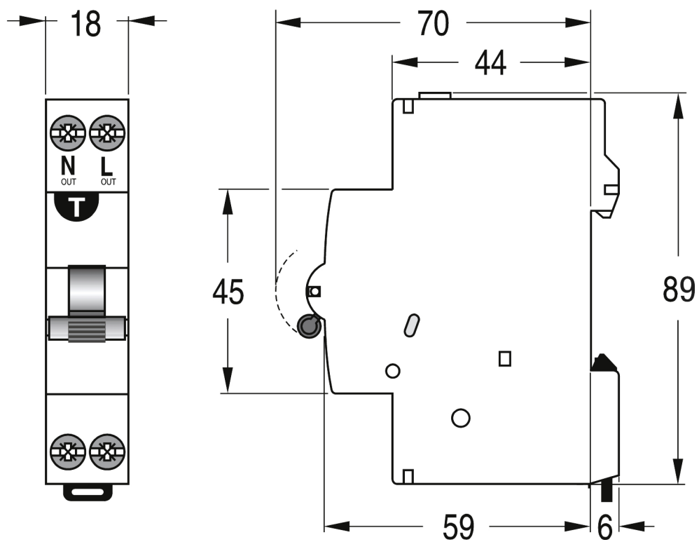
Dimension Diagram
