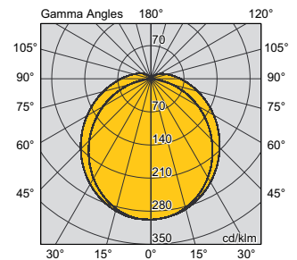
SYMMETRICAL 120°
