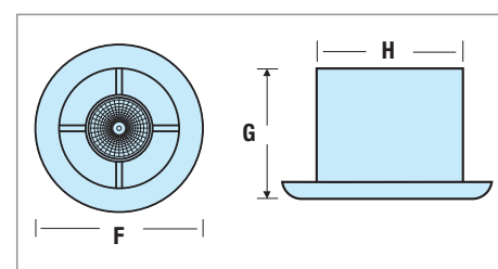
► Dimensions - EL Extract-a-lite Diffuser
