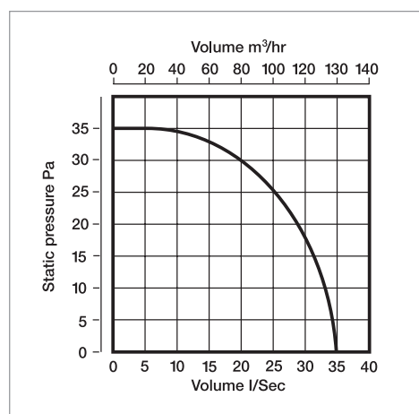
Performance - XPLP125
