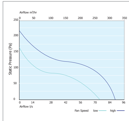
▶ Performance - MF125
