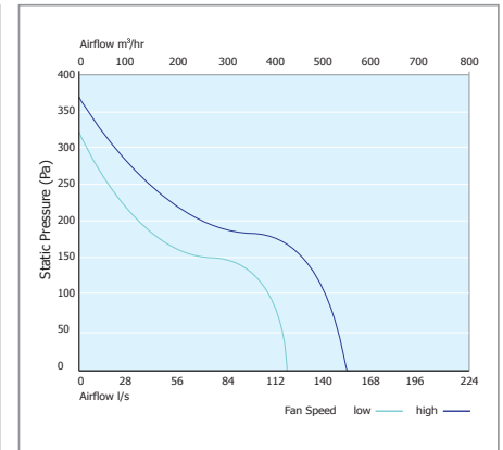
▶ Performance - MF150
