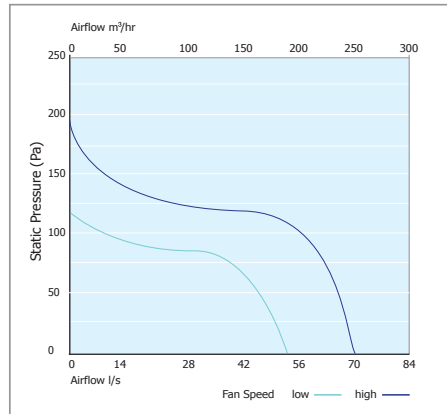
▶ Performance - MF100
