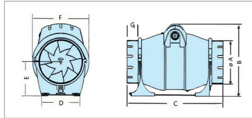
▶ Dimensions - MF
