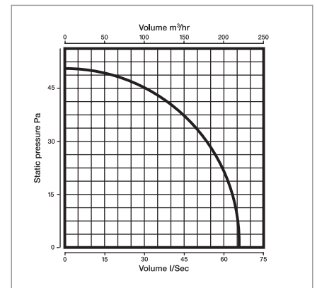
Performance - ECO150
